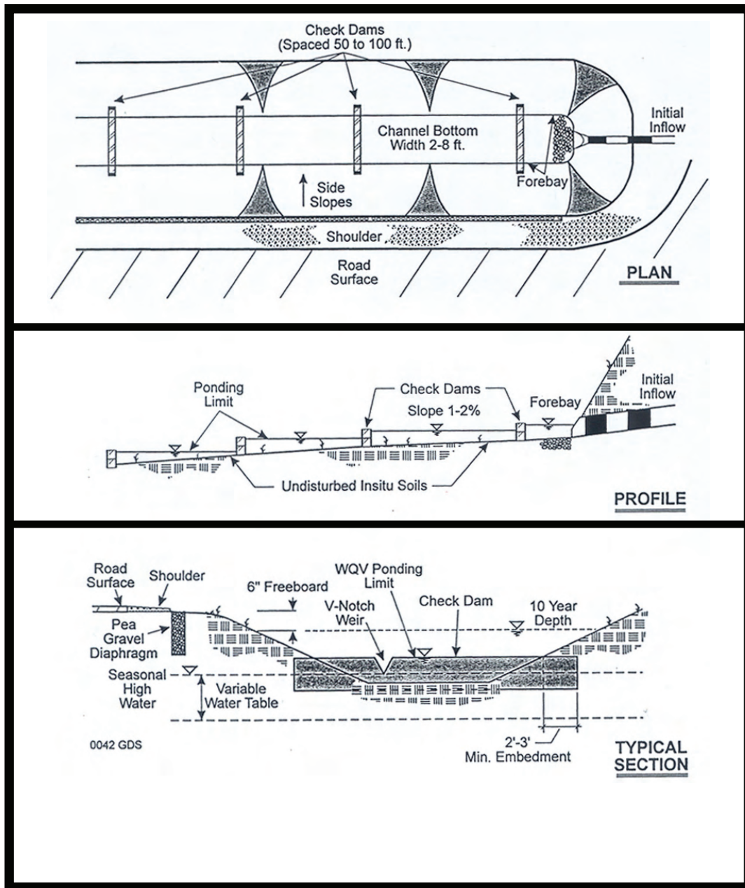
FIGURE 8.13 - Wetland Swale Plan and Profile Example (for informational purposes only)
