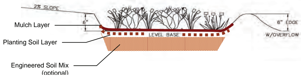
Typical Rain Garden Cross Section (Source: Pennsylvania Stormwater BMP Manual, 2005)
