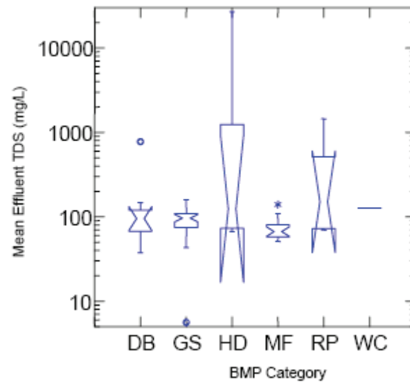
Figure 1. Mean effluent TDS concentration by BMP category
