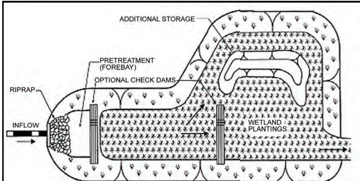
FIGURE 8.14 - Wetland Swale (source: Minnesota Urban Small Sites BMP Manual)
