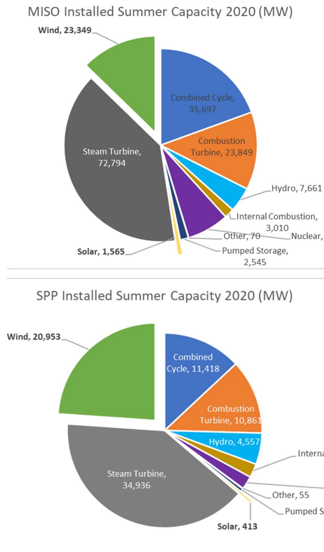
Figure 85: Installed Summer Capacity in MISO and SPP
