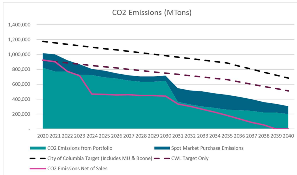
Figure 56: CWL Emission Reductions – Mid Renewable with High CO2 (First Plan)
