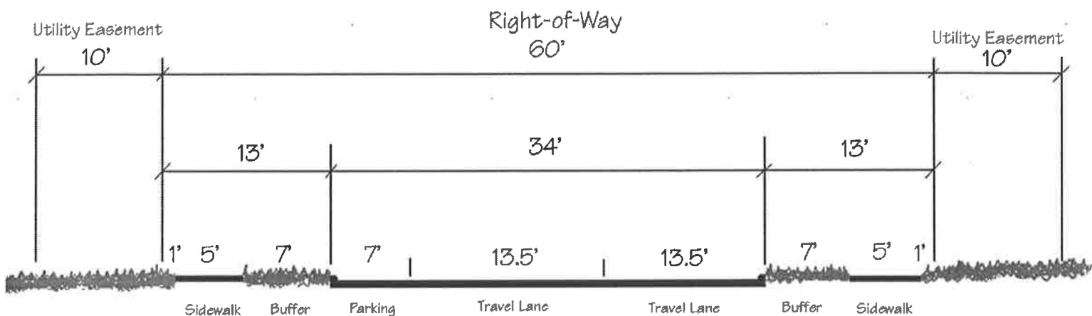
Neighborhood Collector 'Option A'
