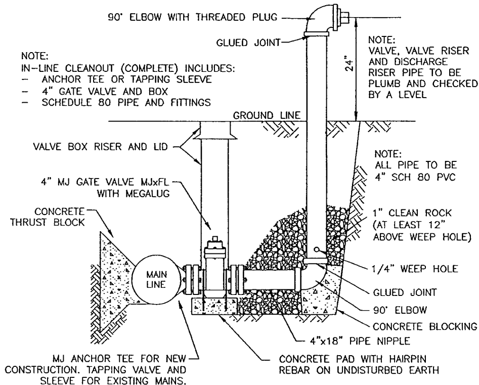
4" SIDE CLEANOUT
