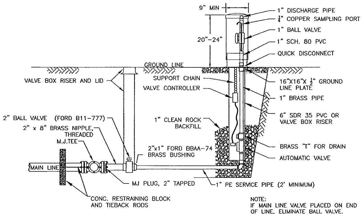
SECTION VIEW
