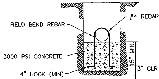
HAIRPIN REBAR DETAIL
