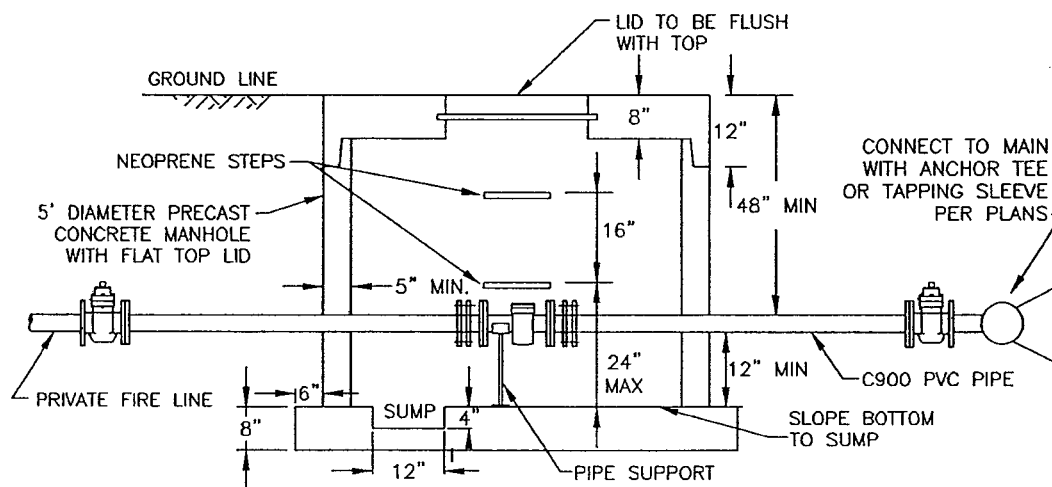
SECTION VIEW
