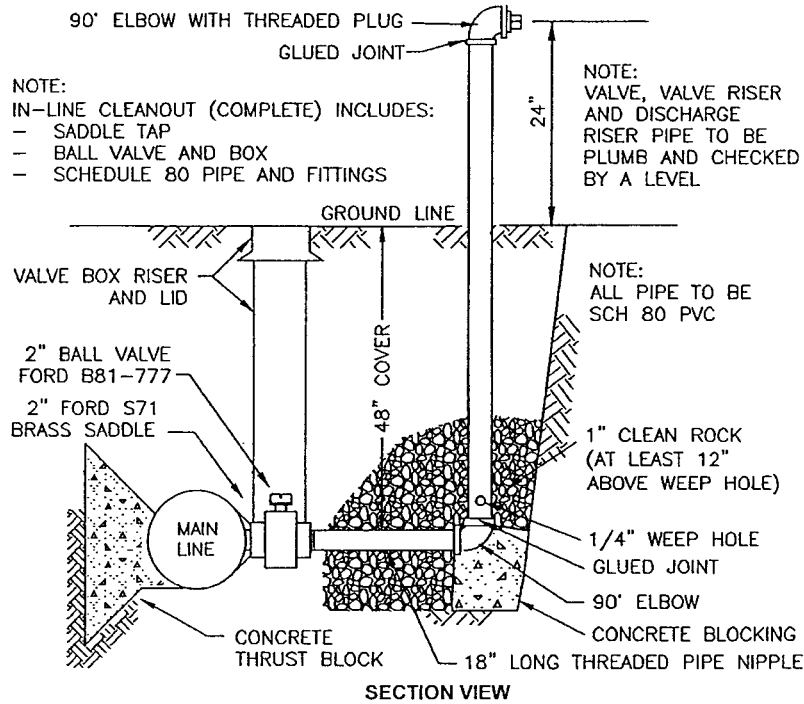
2" SIDE CLEANOUT
