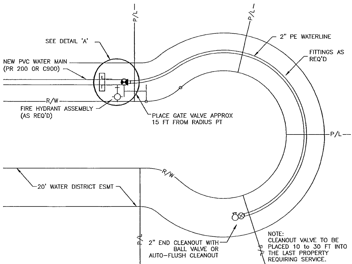
PLAN VIEW
