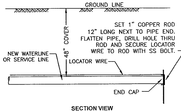
TERMINATION DETAIL
